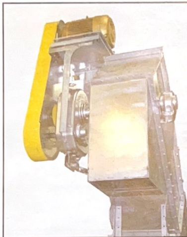
Easy access top motor mount and enclosed belt guard
